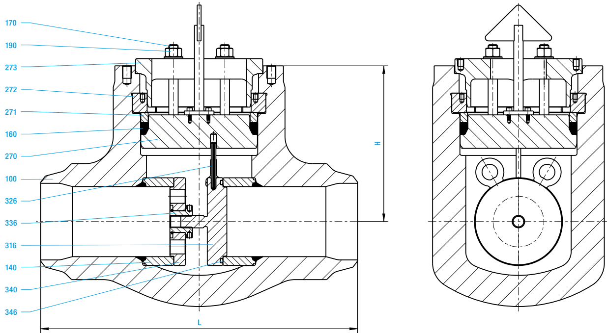
High pressure line blind valve with insert
