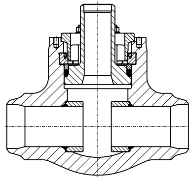
High pressure line blind valve with blow-out insert
